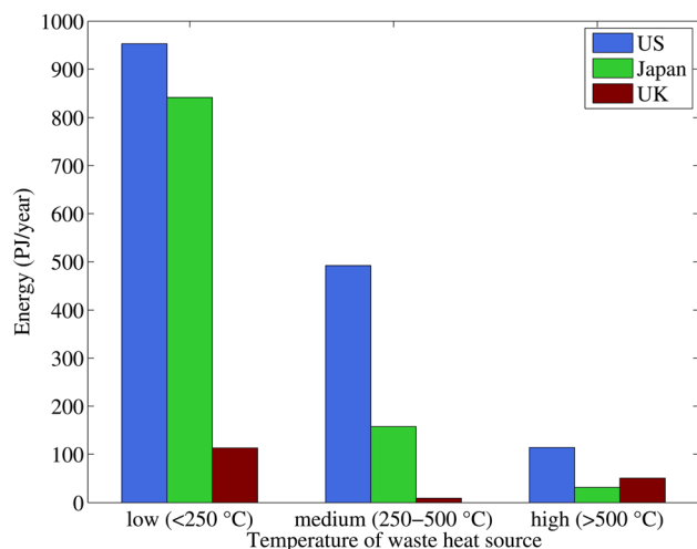
Fig. 6 Annual industrial waste heat in the U.S. [124], Japan [125], and UK [126]. The data are not strictly homogeneous and are shown here together to indicate that the potential for useful conversion is in any case large.
