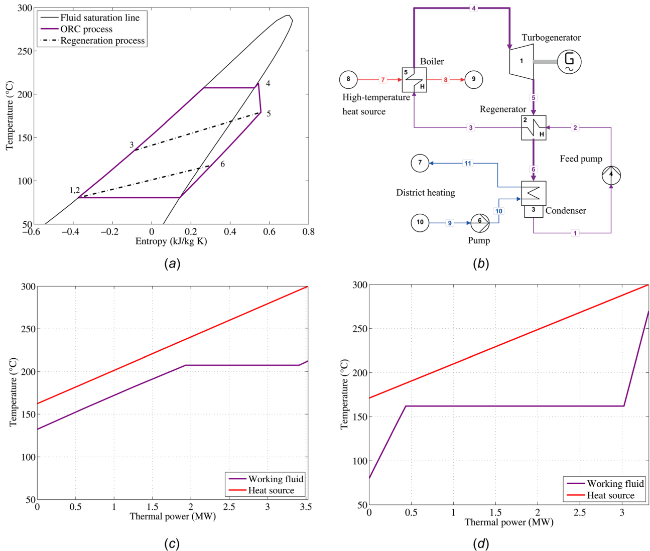
Fig. 1 The processes forming an exemplary superheated/regenerated ORC power plant in the T-s thermodynamic plane of the working fluid, see also Table 5, (a) together with the corresponding process flow diagram (b). (c) Q-T diagram of the evaporator of the ORC system, assuming that the energy source is flue gas at 300^\circ\text{C} , compared to the Q-T diagram of the boiler of a simple steam power plant (d) having flue gas in the same conditions as energy input. The thermodynamic cycles of the ORC and steam power plants have been optimized for maximum net power output having the evaporation pressure and turbine inlet temperature (TIT) as optimization variables, subject to a constraint on the same minimum pinch point in the evaporator (a minimum superheating of 5^\circ\text{C} is also imposed). The main cycle parameters are reported in Table 1.
