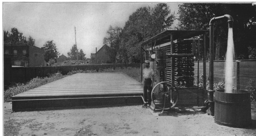
DIRECT ACTING SOLAR ENGINE
