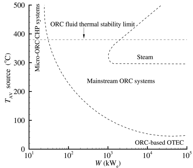
Fig. 2 Current and future fields of application of ORC versus steam power systems in terms of average temperature of the energy source and power capacity of the system. Boundaries are indicative and evolving in time. Adapted from Ref. [11].
