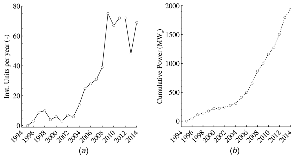
Fig. 4 Number of installed units per year (a) and cumulative power capacity (b) of the commercial ORC power plants commissioned between 1995 and the end of 2013, based on the data reported in Table 3
